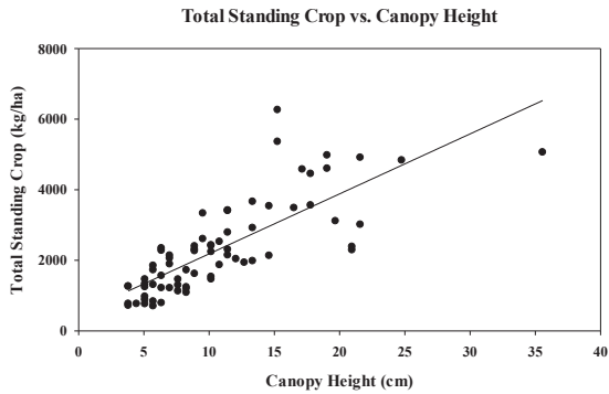
Figure 1 Regression of total standing crop (TSC) on canopy height measured at the 72 field sites 15 September 2014.
