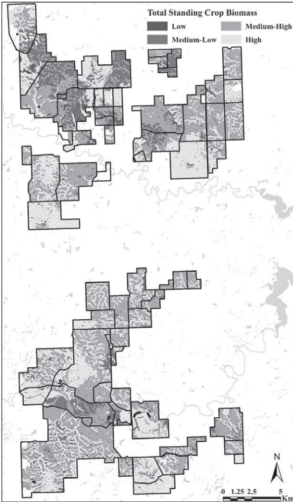
Figure 3 Proportion of landscape that was high, medium-high, medium-low, and low structure in September 2014 according to the TSC-height model thresholds.
