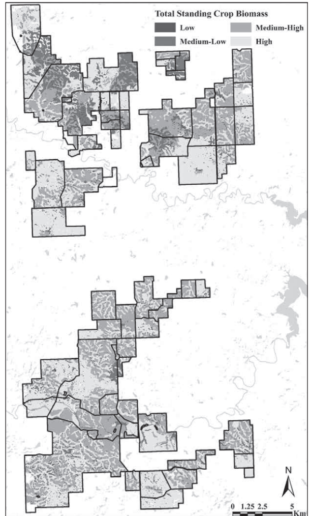
Figure 4 Proportion of landscape that was high, medium-high, medium-low, and low structure in September 2014 according to the TSC-Topo model thresholds.
