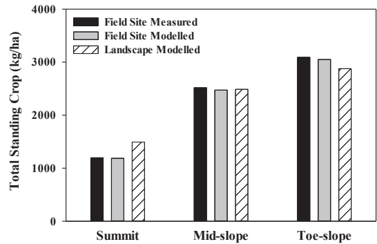
Figure 2 Average (std. error) total standing crop (TSC) measured and modelled at the 72 field sites by topographic position. The hatched bars represent average modelled TSC by topographic position for the entire grassland landscape on 14 September 2014.
