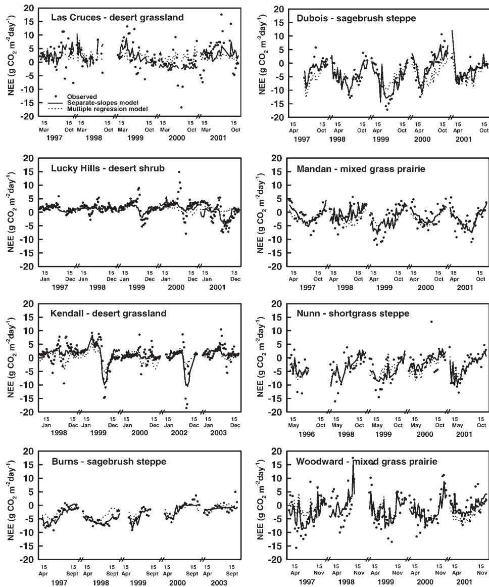
Figure 1. Weekly means of net ecosystem exchange of CO 2 (NEE) for rangeland ecosystems at eight locations in the western United States. Illustrated are data from five growing seasons at each location, including seasons with the greatest and smallest annual total of precipitation. Note that growing season years differ among panels. Dashed lines indicate flux estimates derived from a multiple regression model fit to weekly values of NEE from all years combined. The solid line indicates NEE estimates derived using a regression model in which slopes of significant NEE-environment relationships were allowed to vary among years rather than remain invariant.
