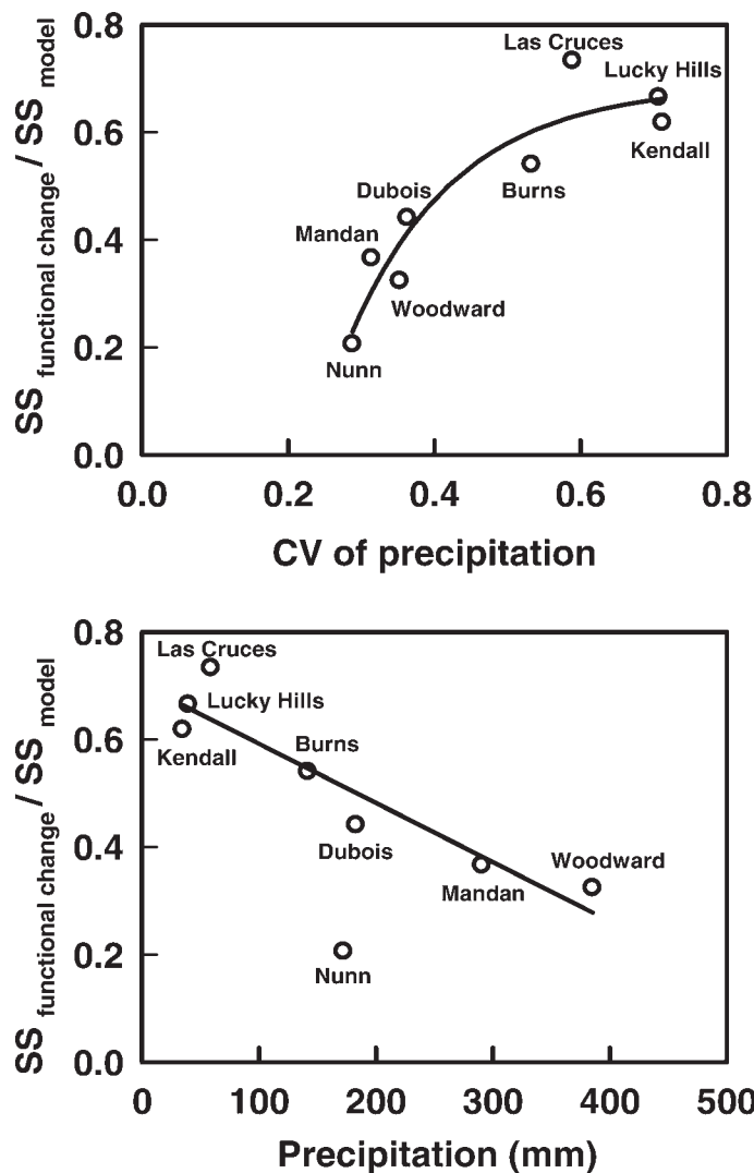
Figure 2. Relationships between the contribution of functional change to the variance in net ecosystem exchange of CO 2 (NEE) explained by a separate-slopes regression model ( SS_{\text{functional change}}/SS_{\text{model}} ) for rangeland ecosystems at each of eight locations and the coefficient of variation (CV) and mean of precipitation, each calculated using precipitation summed through the first one-half of each calendar year of NEE measurements. Lines are exponential and linear regression fits to observations ( r^2 = 0.84 , P = 0.004 and r^2 = 0.86 , P = 0.002 , respectively). Net radiation increases to its maximum value on each rangeland during the first one-half of each year. Physiological activity presumably increases simultaneously. Among-site differences in the variability and amount of precipitation during this period contributed to differences in biotic response functions (functional change) among rangelands.
