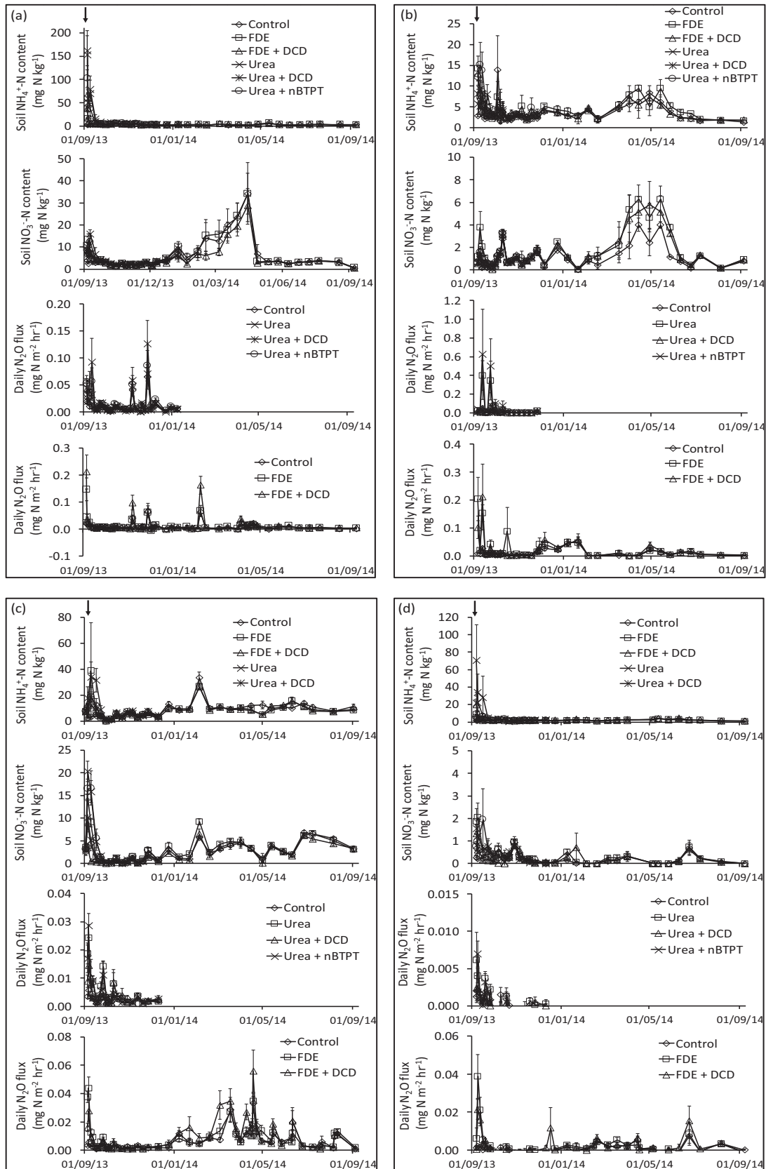
Fig. 3. Soil \text{NH}_4^+\text{-N} , soil \text{NO}_3^-\text{-N} contents and \text{N}_2\text{O} fluxes from 4 sites used for Experiment 1. (a) Waikato, (b) Manawatu, (c) Canterbury and (d) Otago. Solid arrow represents time of fertiliser and FDE application. (Note: different Y axis between experiments).
